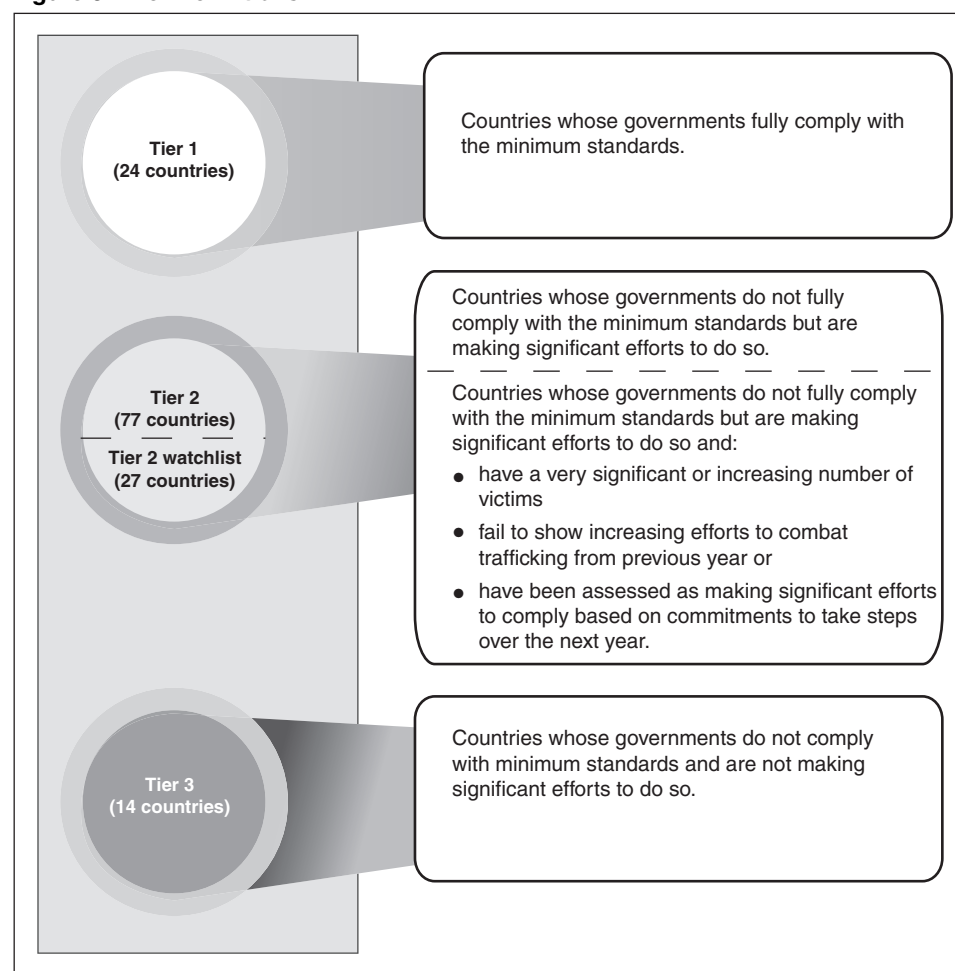
Figure 3: Tier Definitions
